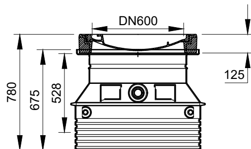
Art.-Nr.:3301.35.12 (Cast iron cover) Art.-Nr.:3301.55.12 (BEGU cover)
