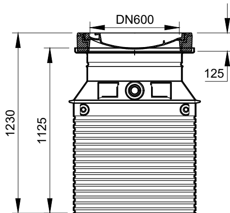
Art.-Nr.:3301.35.13 (Cast iron cover) Art.-Nr.:3301.55.13 (BEGU cover)
