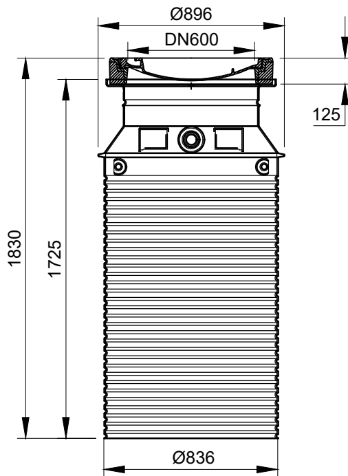
Art.-Nr.:3301.35.13 (Cast iron cover) Art.-Nr.:3301.55.13 (BEGU cover)
