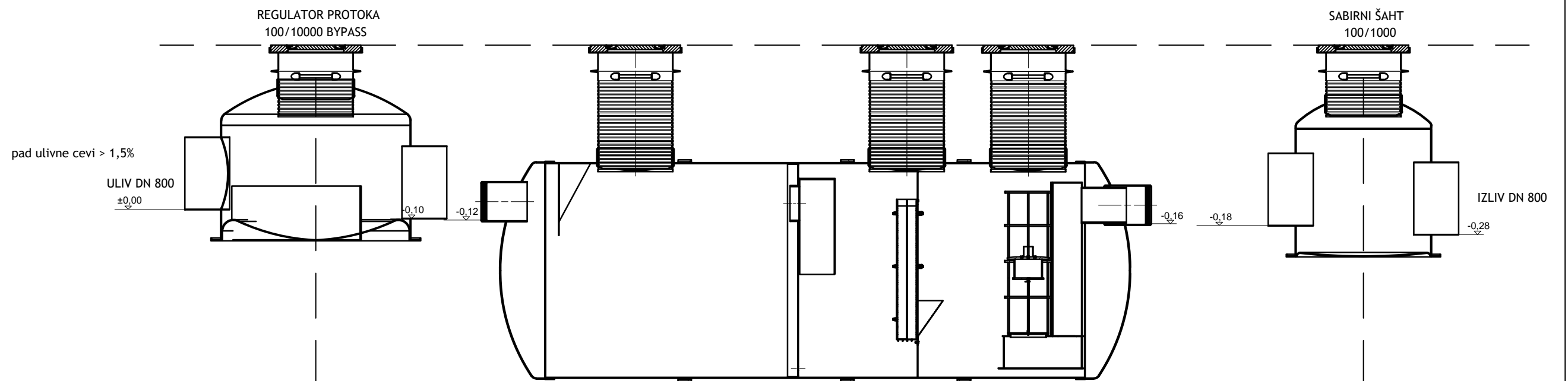
ACO Oleopator-FST-G-H NS100/10000
