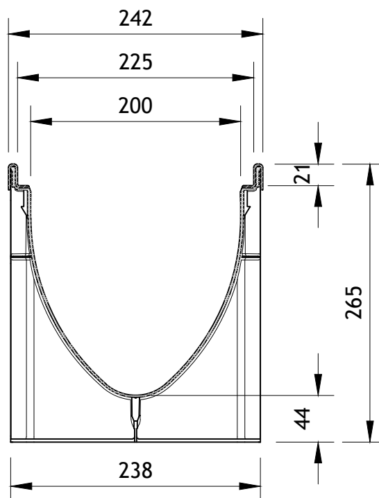
ACO XtraDrain X200S
