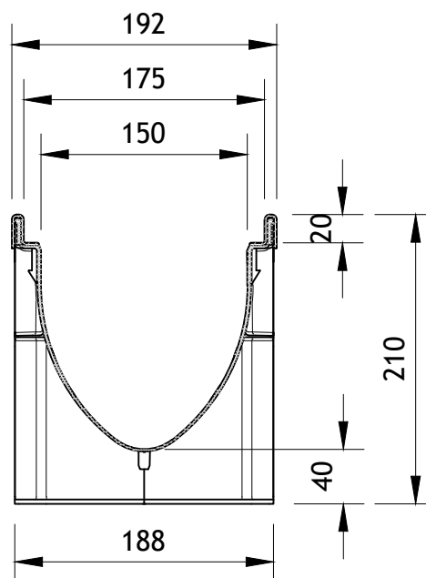
ACO XtraDrain X150S
